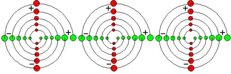
Figure 9: Helical Electromagnetic Waves
