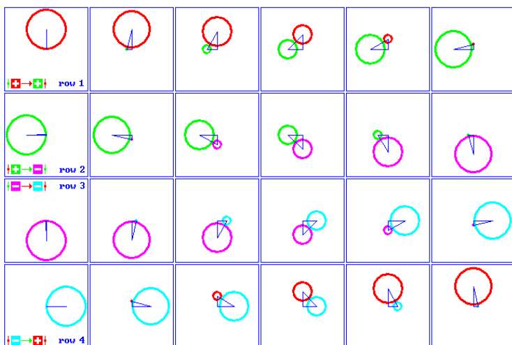
Figure 15: Cross sections through flux tubes
