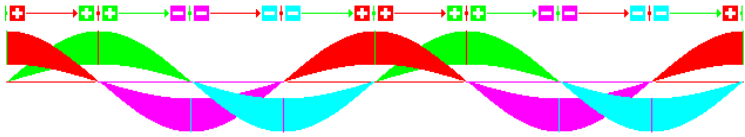
Figure 13: Flux tubes with polarity color
