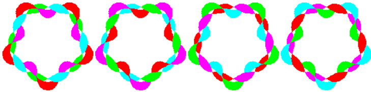
Figure 27: This is loops of light as particles
