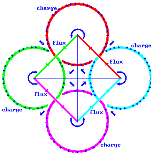
Figure 19: Cross section through flux tubes
