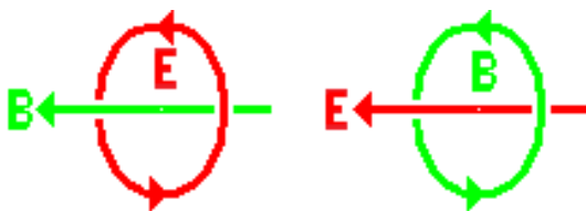
Figure 4: Faraday's and Ampere's Laws
