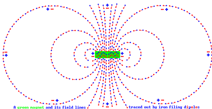
Figure 22: Iron filings and bar magnets
