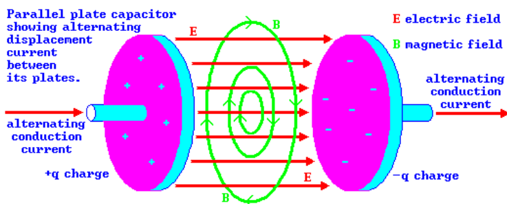
Figure 12: Ampere's law and the electromagnetic wave
