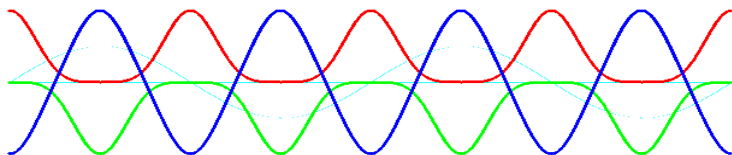
Figure 28: Unimpeded torques of the light wave
