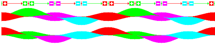
Figure 14: Flux tubes in three dimensions
