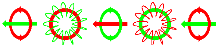
Figure 10: Perpendicular Transformations
