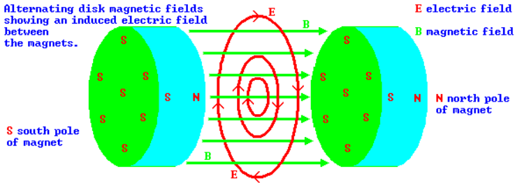
Figure 11: Faraday's law and the electromagnetic wave
