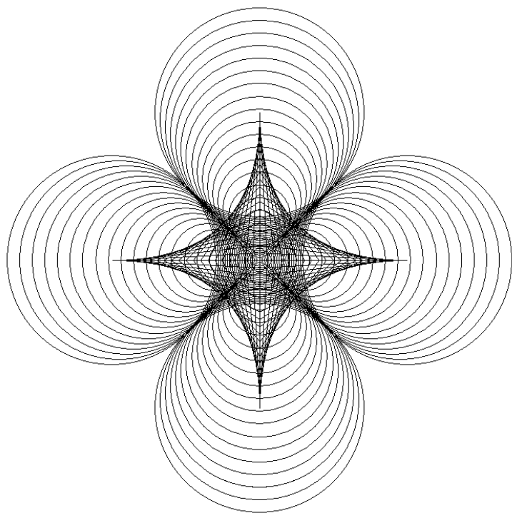
Figure 29: A stack of cross sections through the electromagnetic wave
